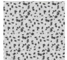
TYPICAL CONTAMINANT DIMENSION IN A HYDRAULIC CIRCUIT (4-14 \mu\text{m} )
